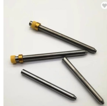
Waterjet Cutting Parts Nozzle Mixing Tubes 7.14*1.02*76.2mm
