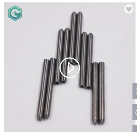
7.14*1.02*76.2mm waterjet cutting machine parts waterjet abrasive nozzle mixing tube
