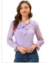
Airy H Line...
