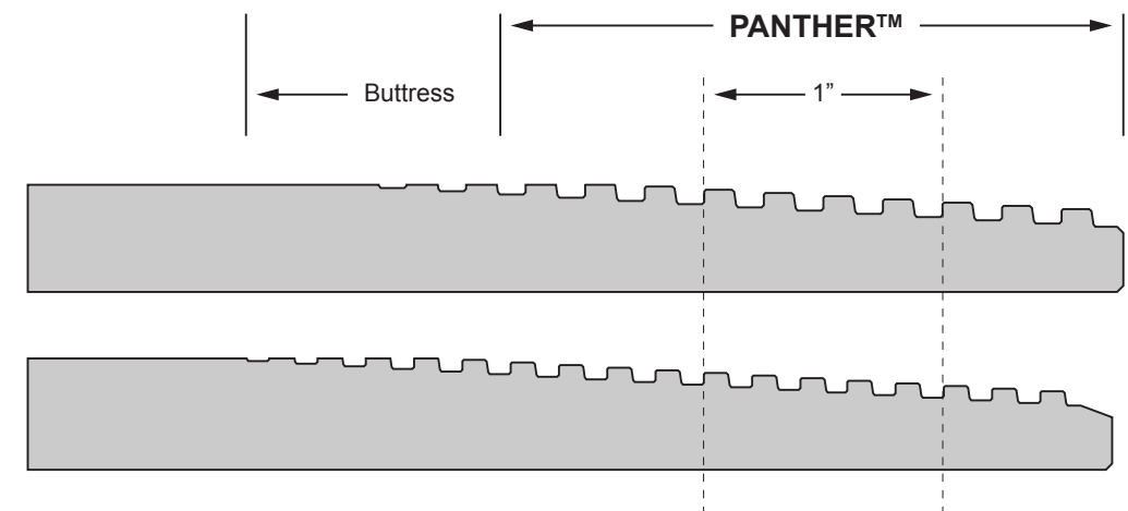
Compared to 5 pitch buttress style connections, the PANTHER™ steep taper and reduced thread pitch is easy and dependable to run.
