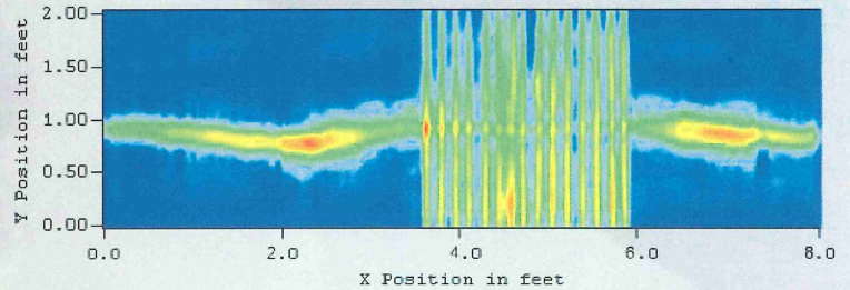
Mapping post tension cable and rebar
