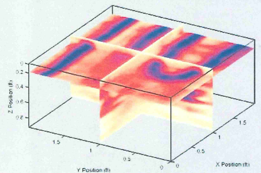
Locating radiant heating tubes
