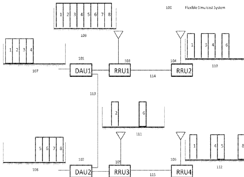
Flexible Simulcast Downlink Example
