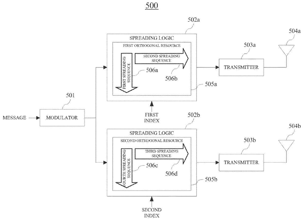
FIG. 5 (PRIOR ART)
