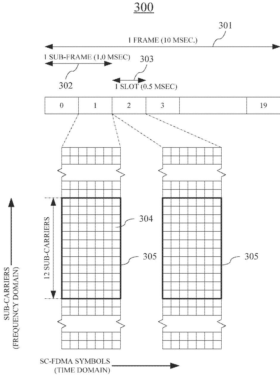
FIG. 3 (PRIOR ART)
