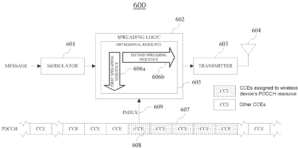
FIG. 6 (PRIOR ART)
