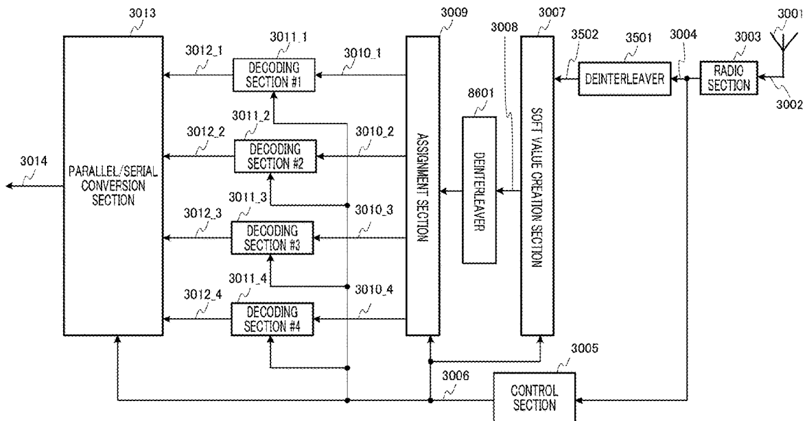
8600 RECEIVING APPARATUS
