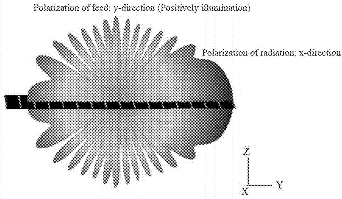
FIG. 7 (c) Space waves illuminated obliquely (Array of slots)
