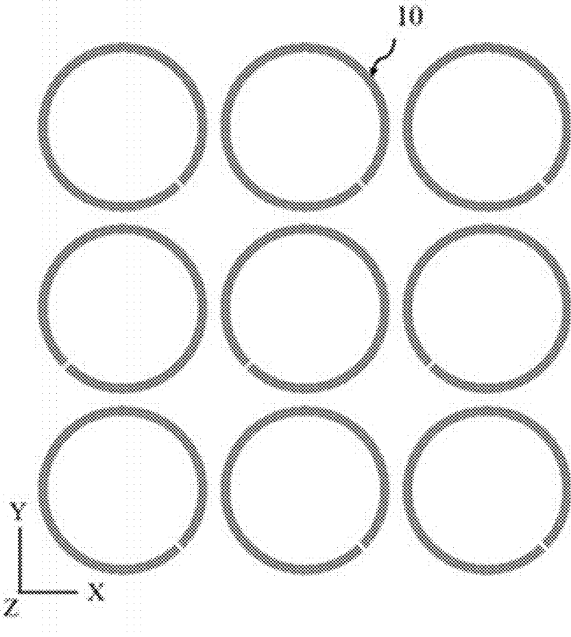
FIG. 6 (b) Partial enlargement view - Array of dipoles
