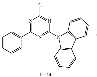
[Reaction Scheme 3]
