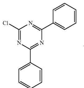
[Reaction Scheme 4]
