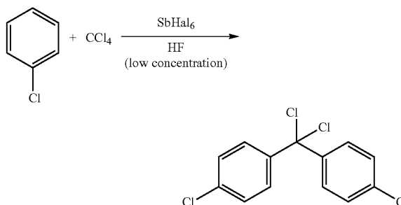
Scheme 1: Friedel-Crafts reaction with \text{CCl}_4 (one pot) batch or continuous (inventive procedure).
