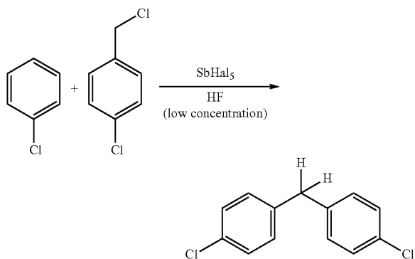
Scheme 3: Friedel-Crafts reaction with 4-chloro-1-(chloromethyl)benzene, for preparing dichlorodiphenylmethane, batch or continuous (inventive procedure).
