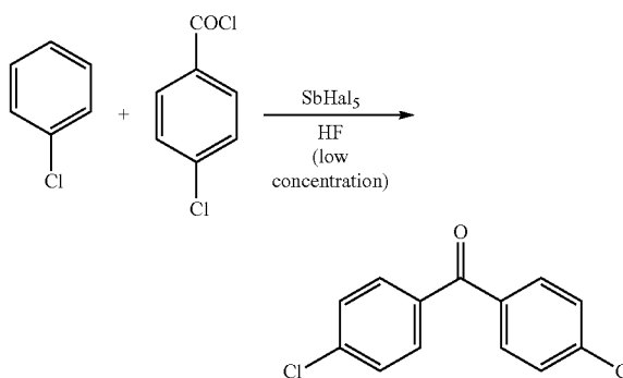
Scheme 2: Friedel-Crafts reaction with 4-chlorobenzoyl chloride, (one pot) batch or continuous (inventive procedure).
