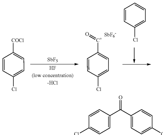
Scheme 5: Acylation of chlorobenzene according to the invention.
