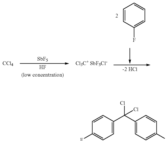
Scheme 6: Acylation of fluorobenzene according to the invention.
