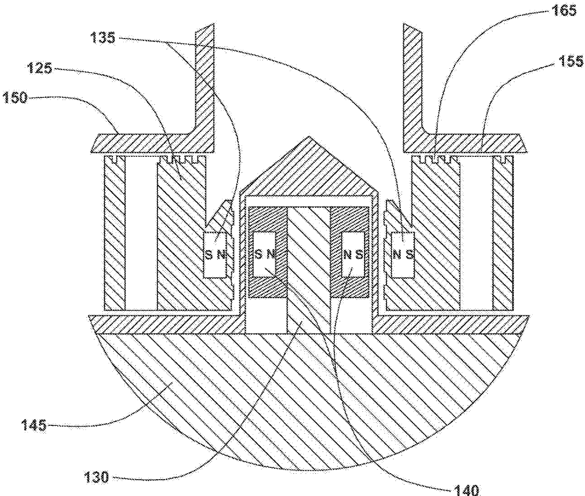
FIG. 13 (DETAIL D)
