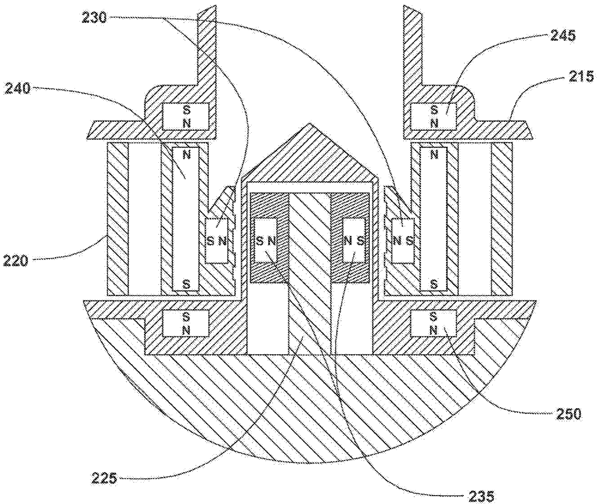
(DETAIL H)
