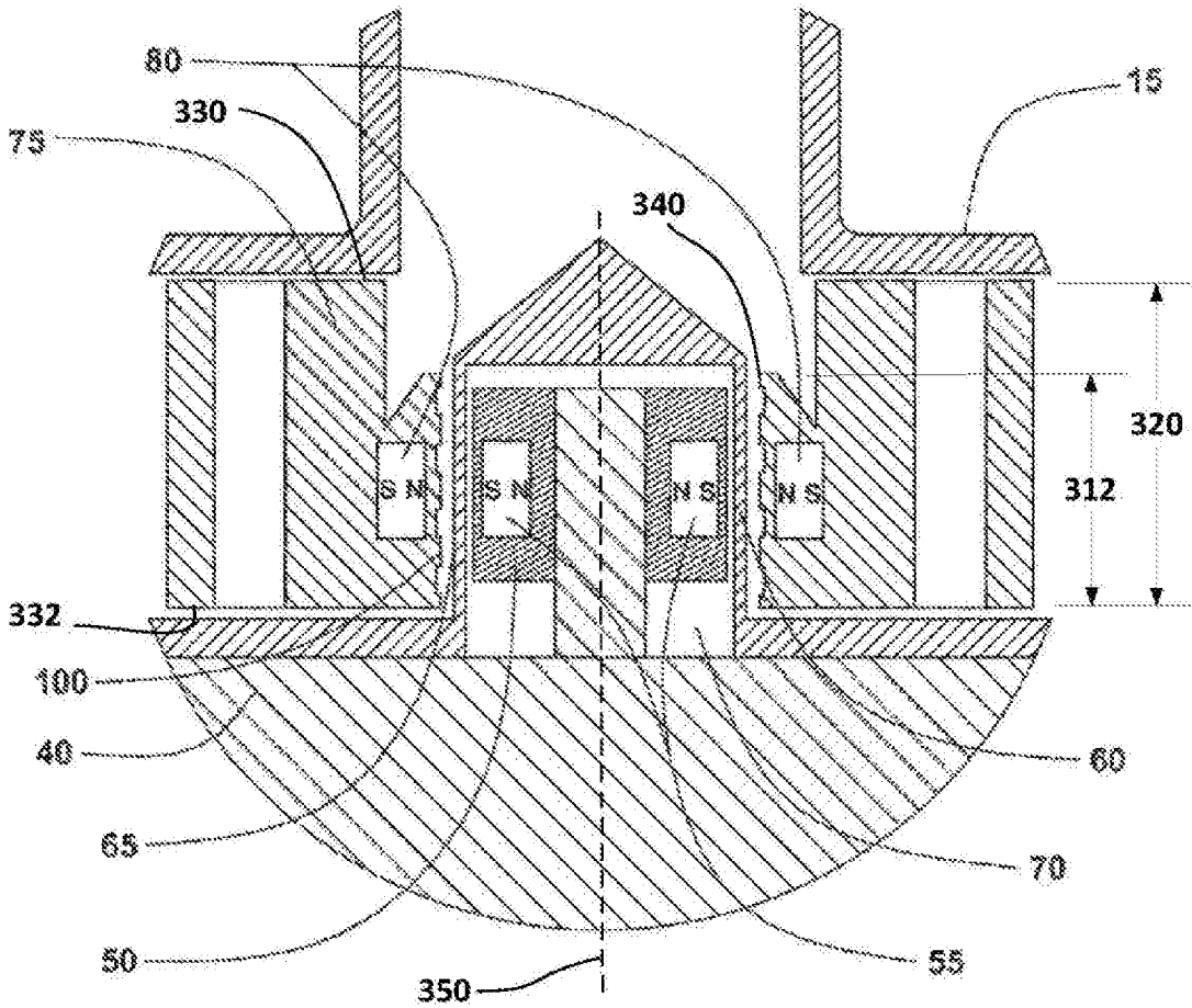
FIG 4 (DETAIL C)
