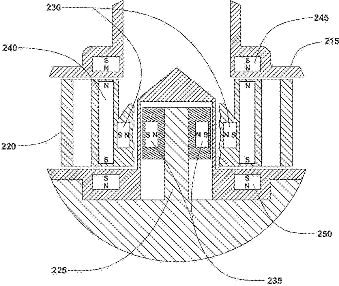
FIG.20 (DETAIL H)
