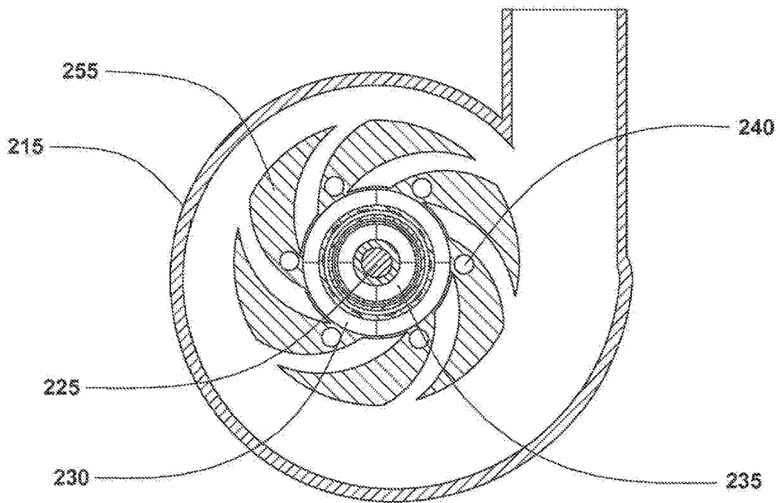
FIG. 19 (Section G-G)
