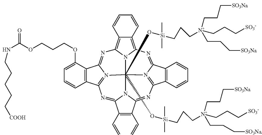
[Chemical Formula 8]
