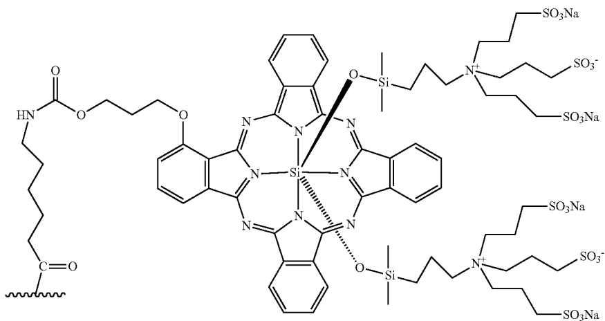
[Chemical Formula 4]
