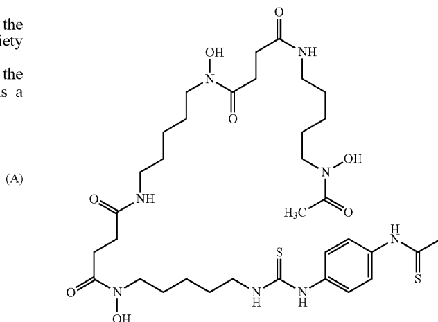
[Chemical Formula 11]
