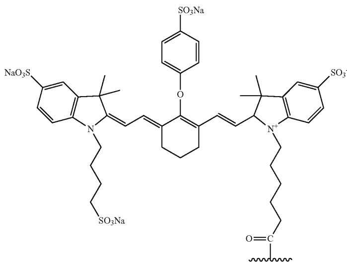
[Chemical Formula 12]
