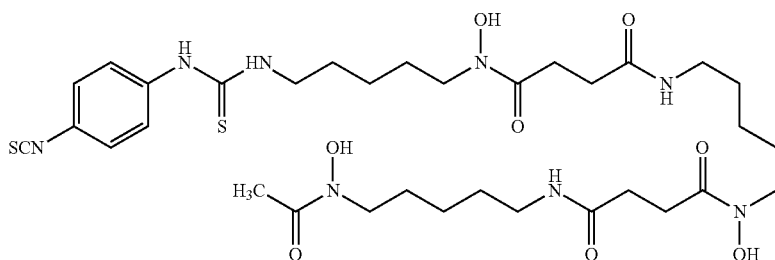
[Chemical Formula 9]
