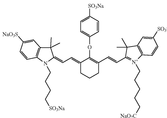
[Chemical Formula 7]
