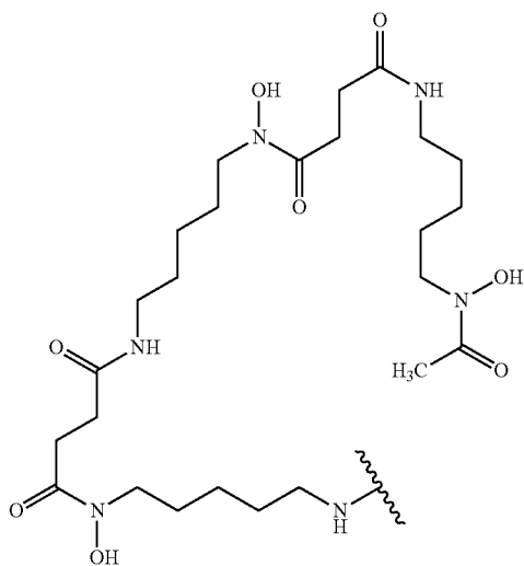
[Chemical Formula 10]
