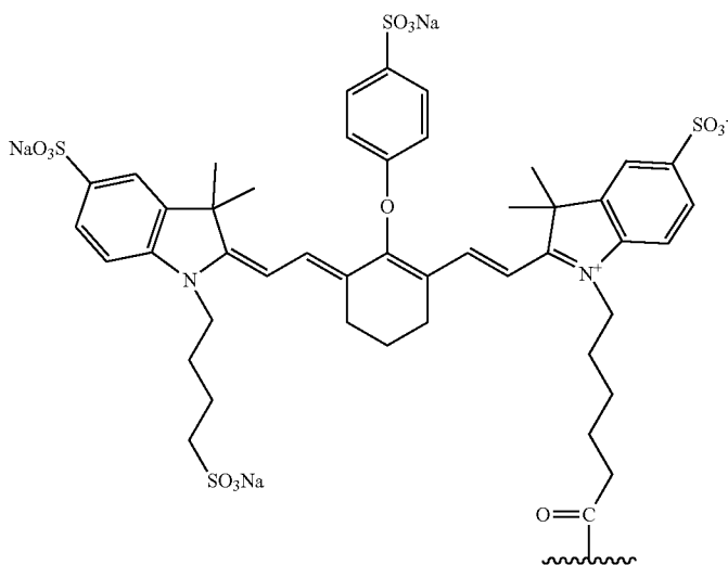
[Chemical Formula 4]
