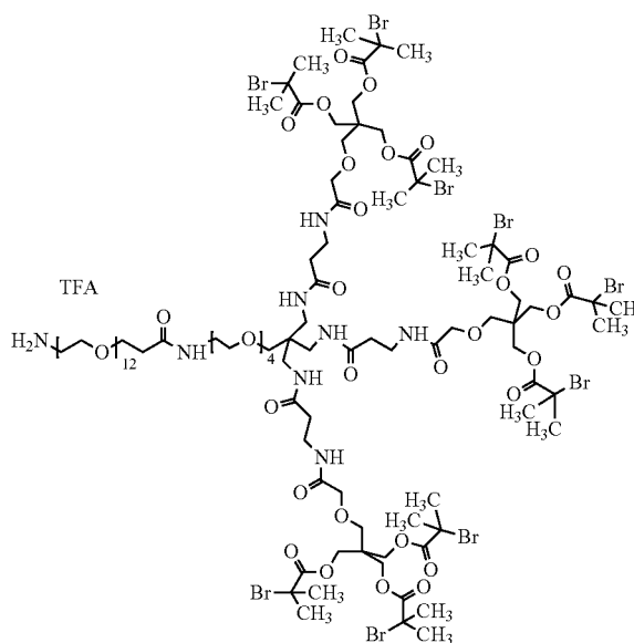
Compound P
