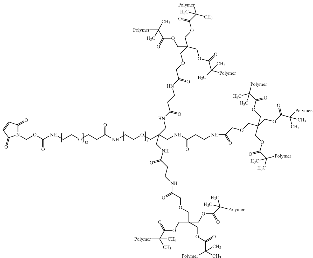
Polymer R
