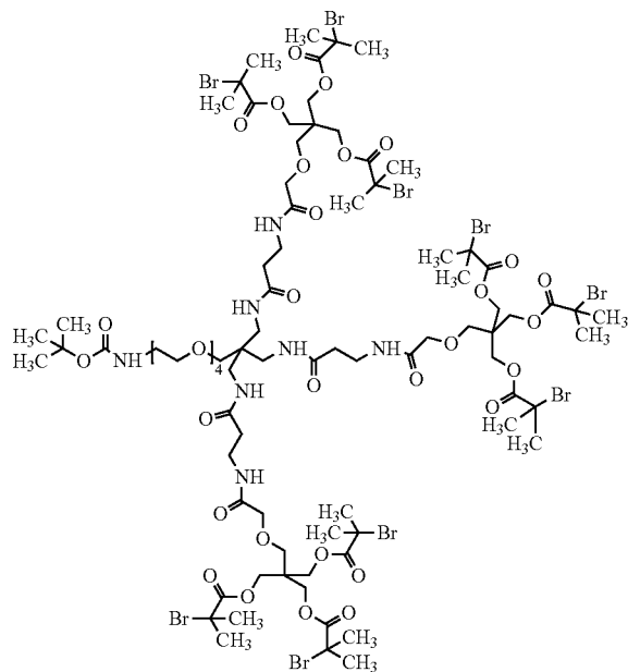
Compound K
