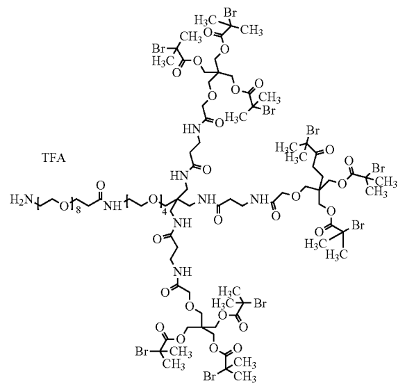
Compound O
