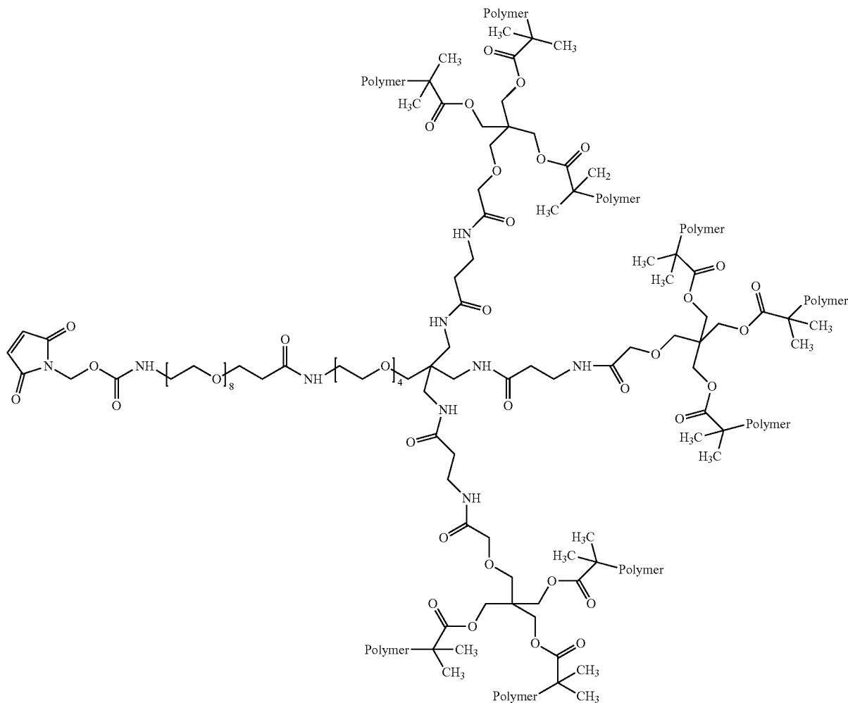
Polymer Q
