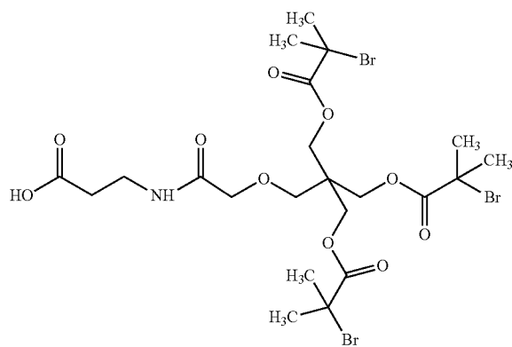
Compound J
