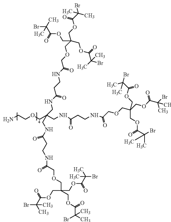
Compound L
