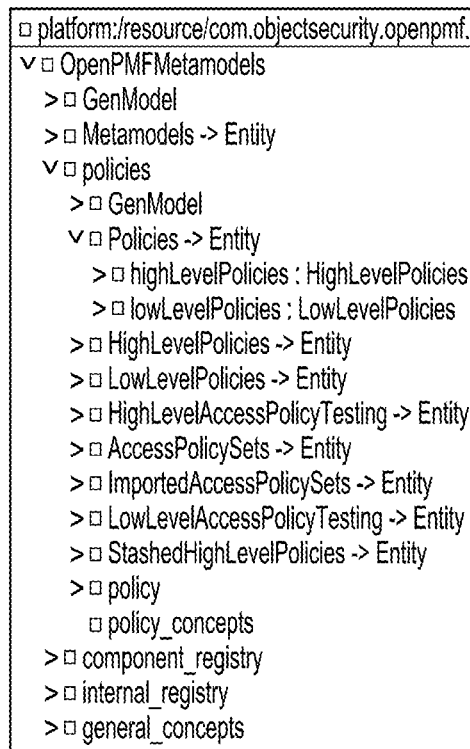
Example metamodel (excerpt)
