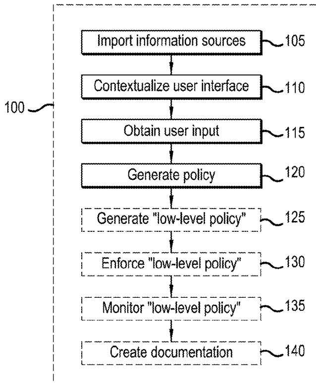
Assisted policy management example steps
