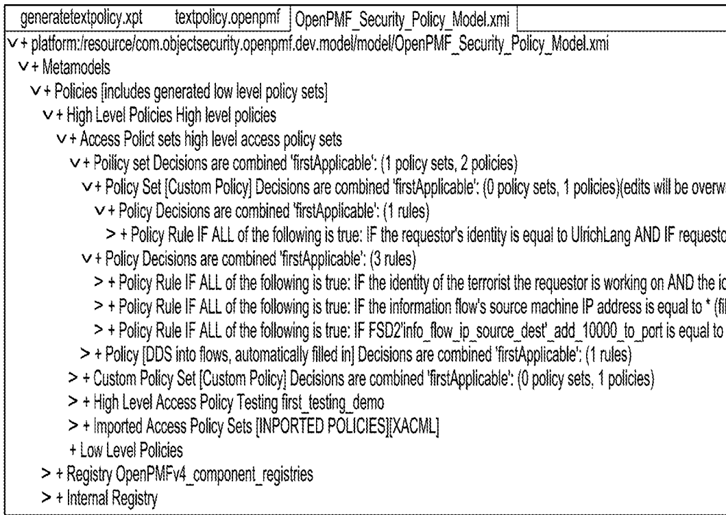
Example data model based on metamodel (excerpt)
