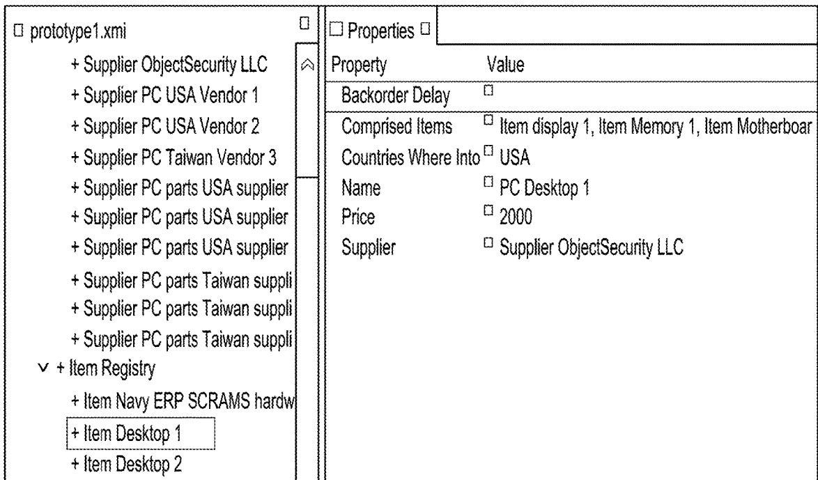
SCRAMS example item properties
