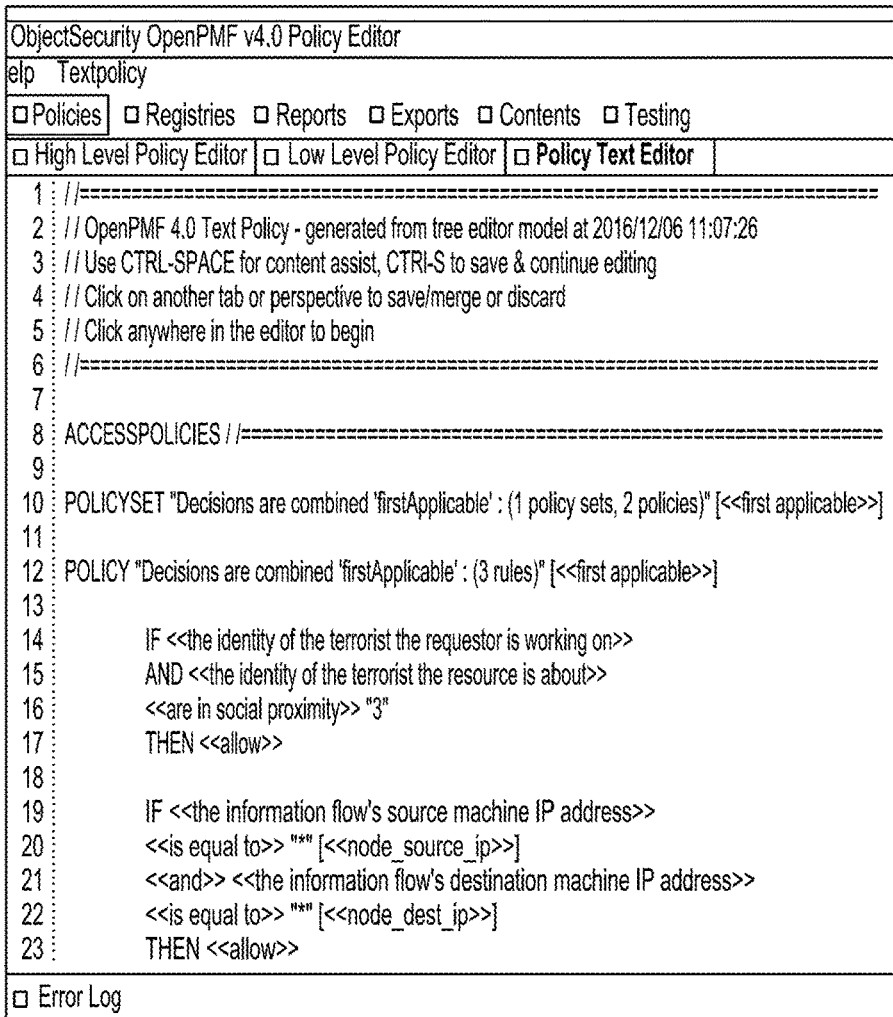
Example textual editor FIG.3B
