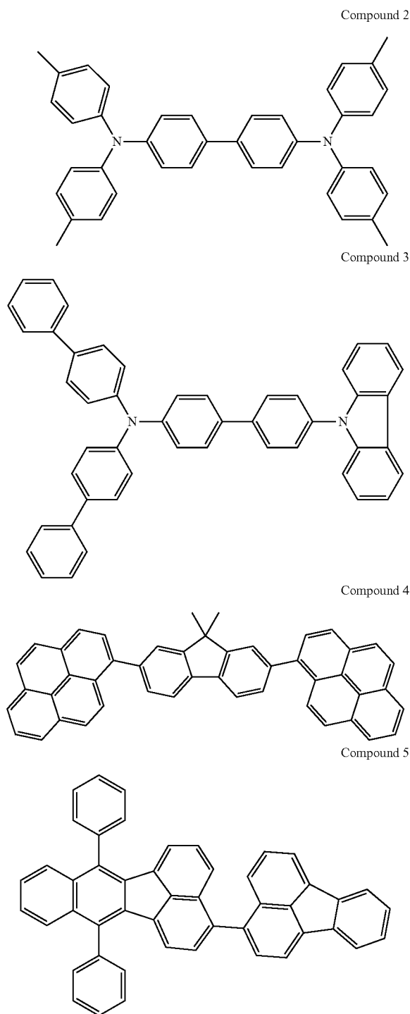
Compound 2
