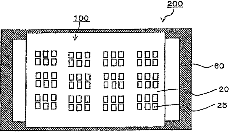
VIEW SEEN FROM RESIN MASK SIDE
