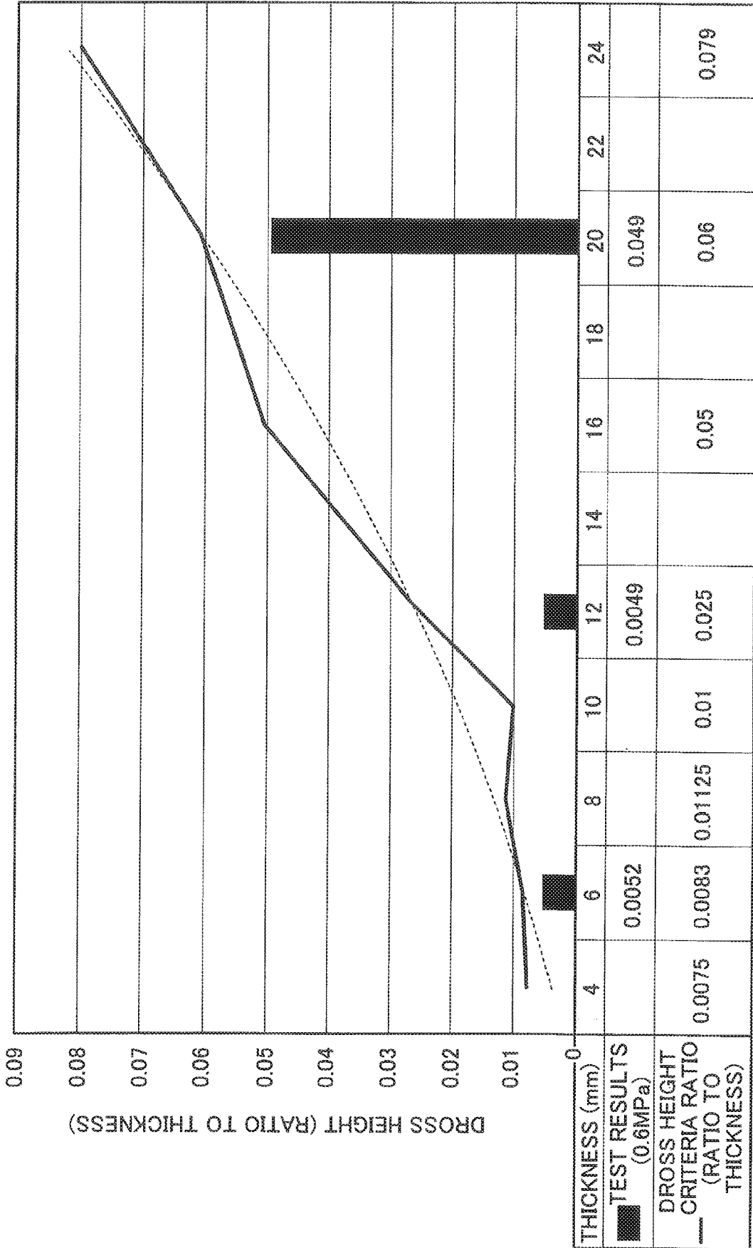
FIG. 3 DROSS HEIGHT CRITERIA (CUTTING PERFORMANCE EVALUATION CRITERIA)
