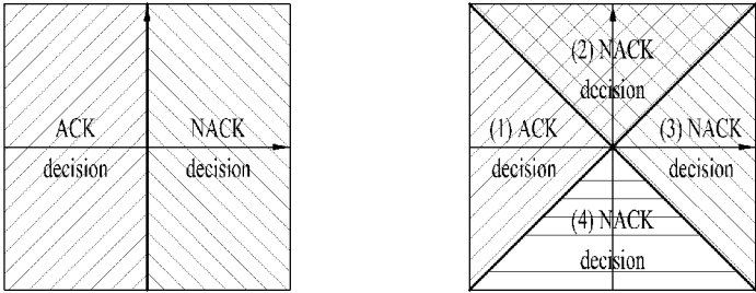
(a) Conventional 1-bit ACK/NACK decision region
