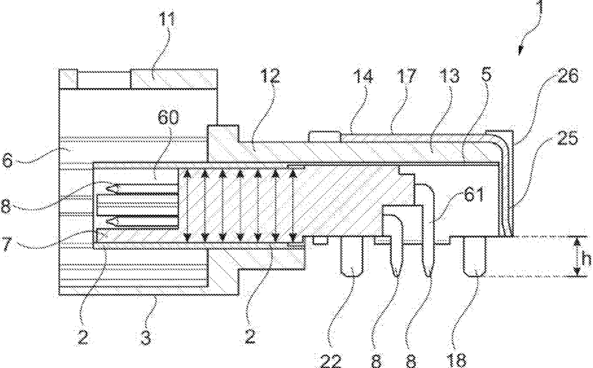
Fig. 3 PRIOR ART
