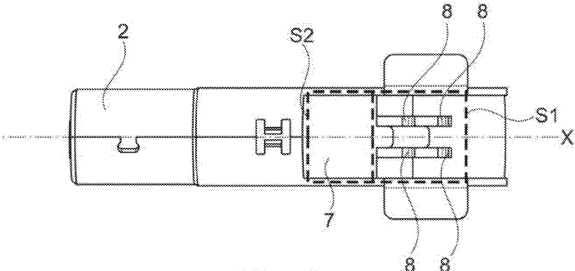
Fig. 4 PRIOR ART
