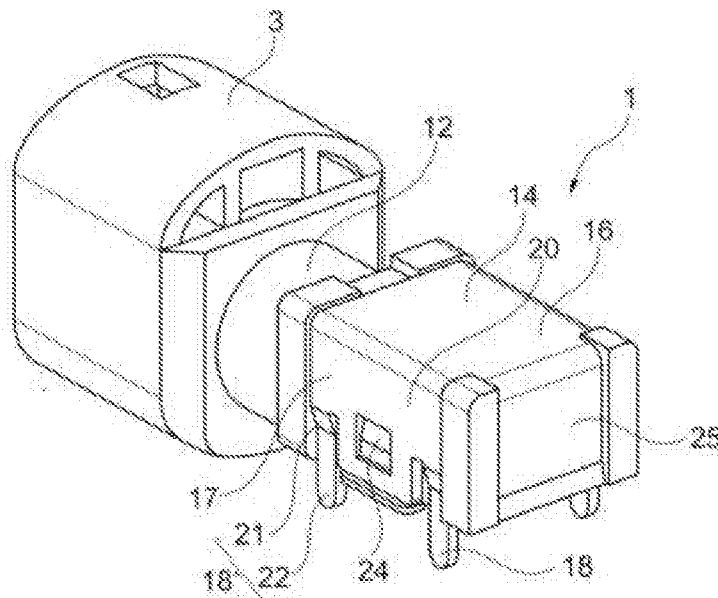
Fig. 2 PRIOR ART
