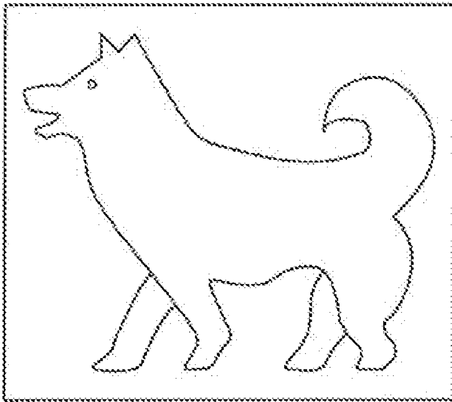
INPUT IMAGE
