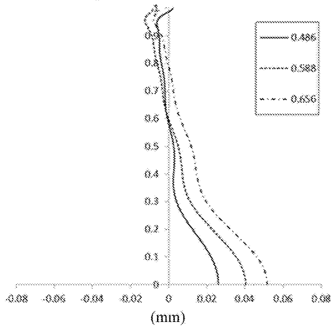
Longitudinal Aberration Curve
