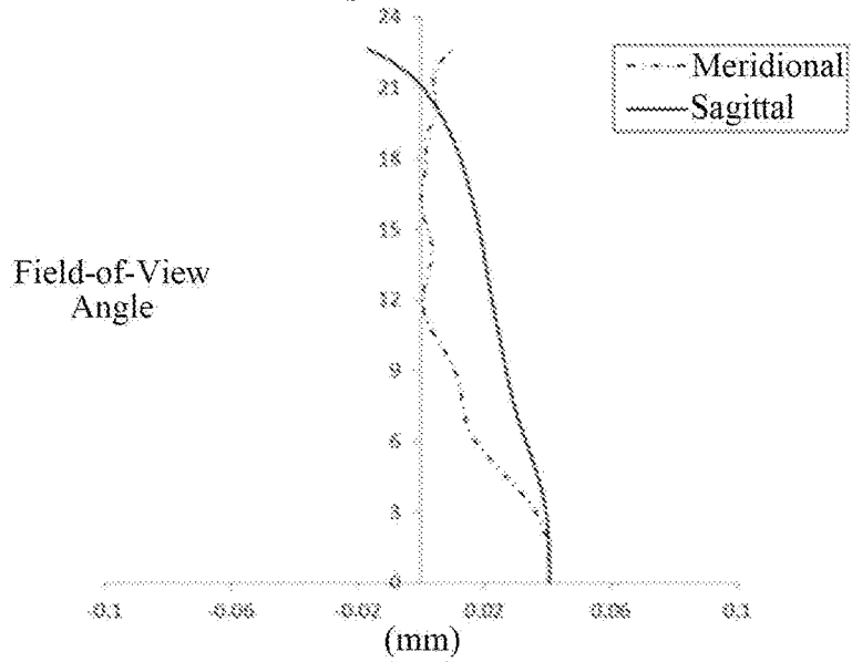
Astigmatism Curve
