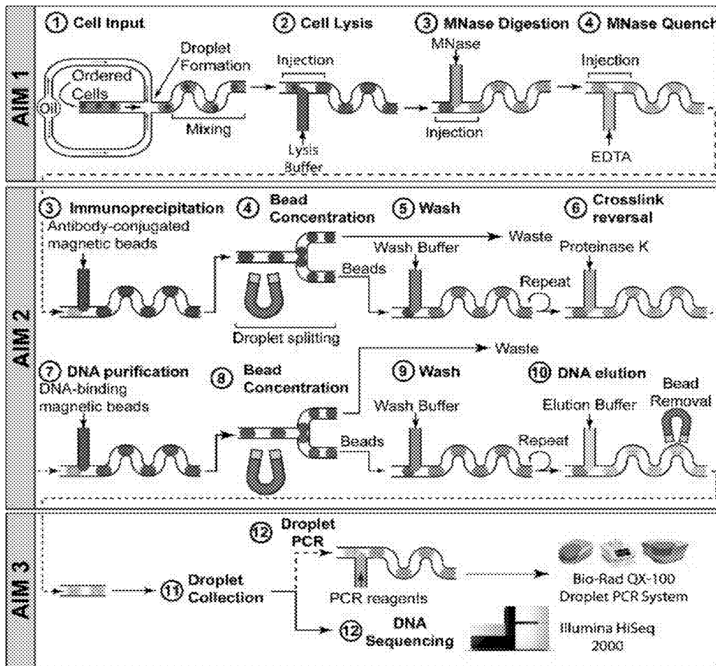
FIG. 1D
