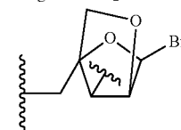
\alpha -L-LNA ( \alpha -L-configuration) bridge = 4'-CH 2 —O-2'
