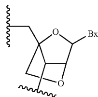
LNA ( \beta -D-configuration) bridge = 4'-CH 2 —O-2'
