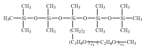
Chemical formula 18
