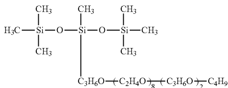
Chemical formula 14
