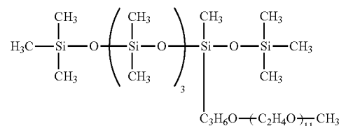
Chemical formula 10
