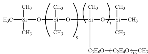
Chemical formula 12
