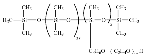
Chemical formula 13
