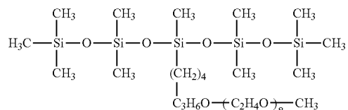
Chemical formula 17
