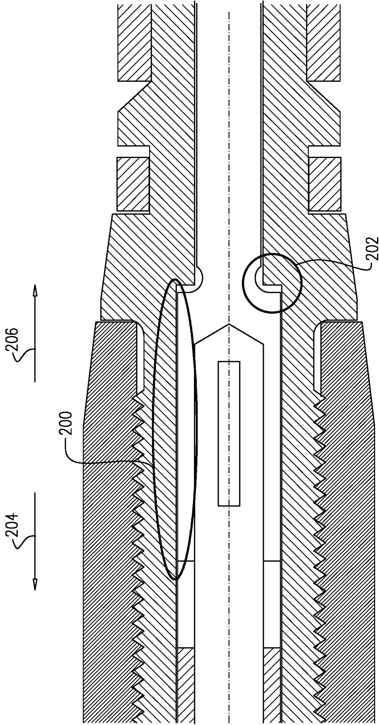
FIG. 5C PRIOR ART
