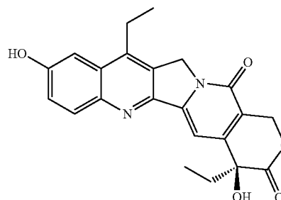
(7-Ethyl-10-hydroxy-camptothecin)
