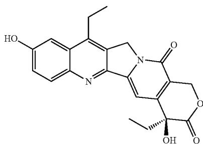
(7-Ethyl-10-hydroxy-camptothecin)
