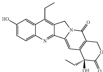
(7-Ethyl-10-hydroxy-camptothecin)
