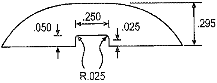
5-WIRE OPENING
