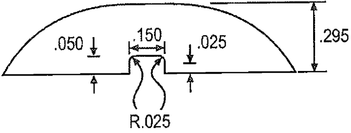
3-WIRE OPENING
