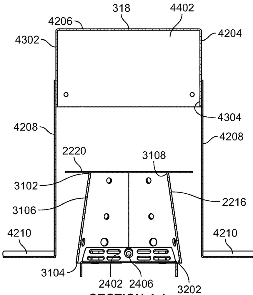
SECTION J-J
