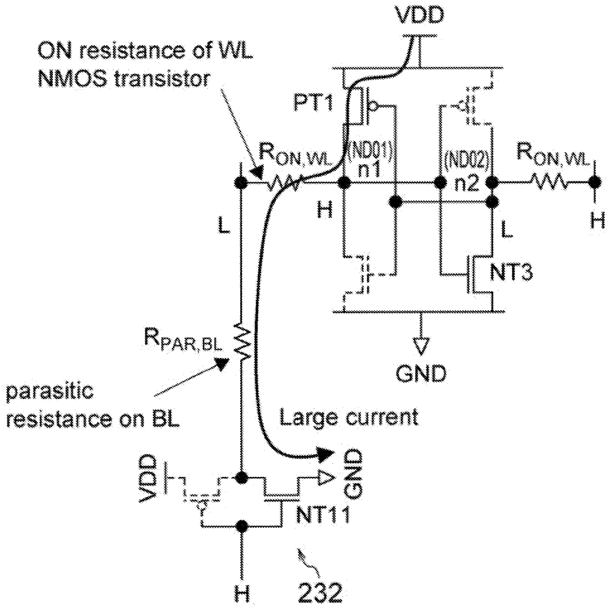
FIG. 11B (Related Art)
