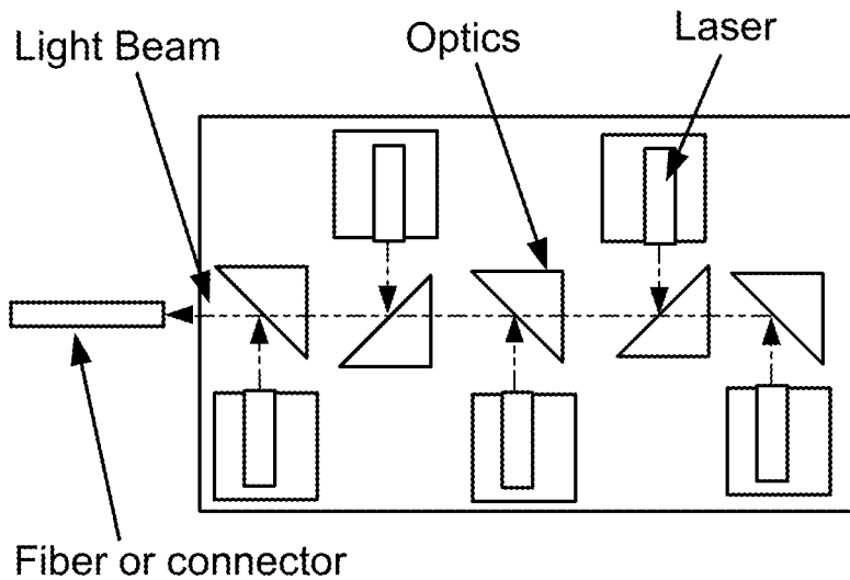
2 row configuration
