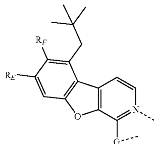
L_{Ai-10} based on Structure 10:
