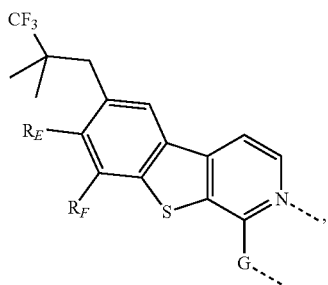
L_{Ai-4} based on Structure 4:
