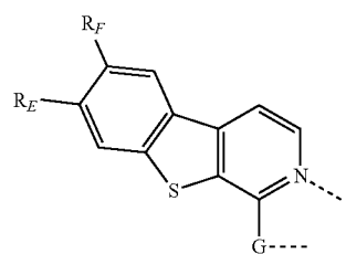
L_{Ai-31} based on Structure 31:
