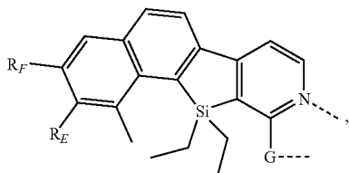
L_{Ai-25} based on Structure 25:
