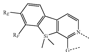
L_{Ai-19} based on Structure 19:
