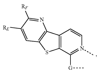
L_{Ai-28} based on Structure 28:
