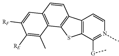
L_{Ai-1} based on Structure 12:
