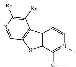
L_{Ai-29} based on Structure 29:
