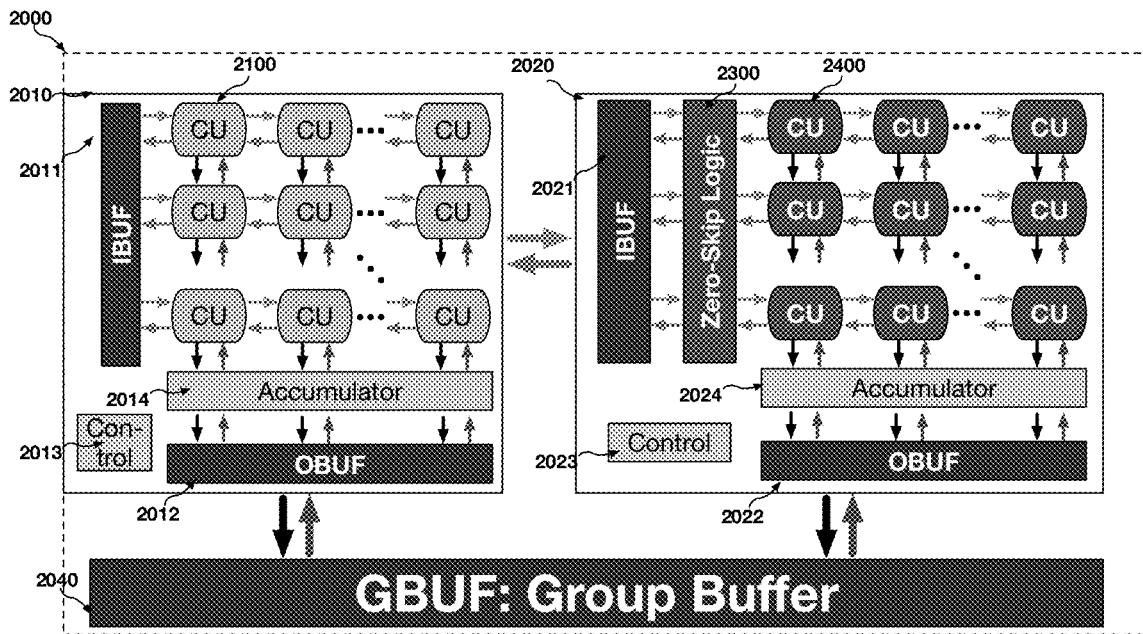
FIG. 17 Proposed architecture for training quantized neural networks.
