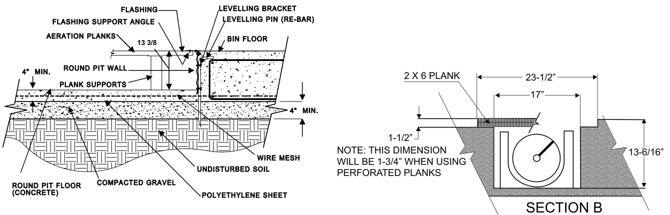
Figure 4. Foundation Plan View and Sectional
