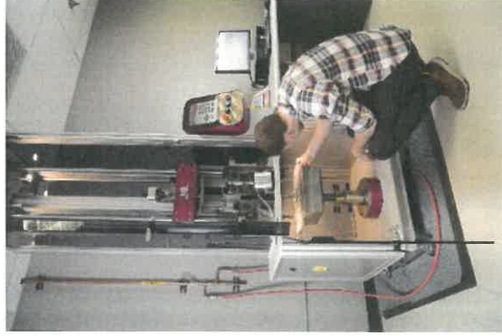
Instron CEAST
